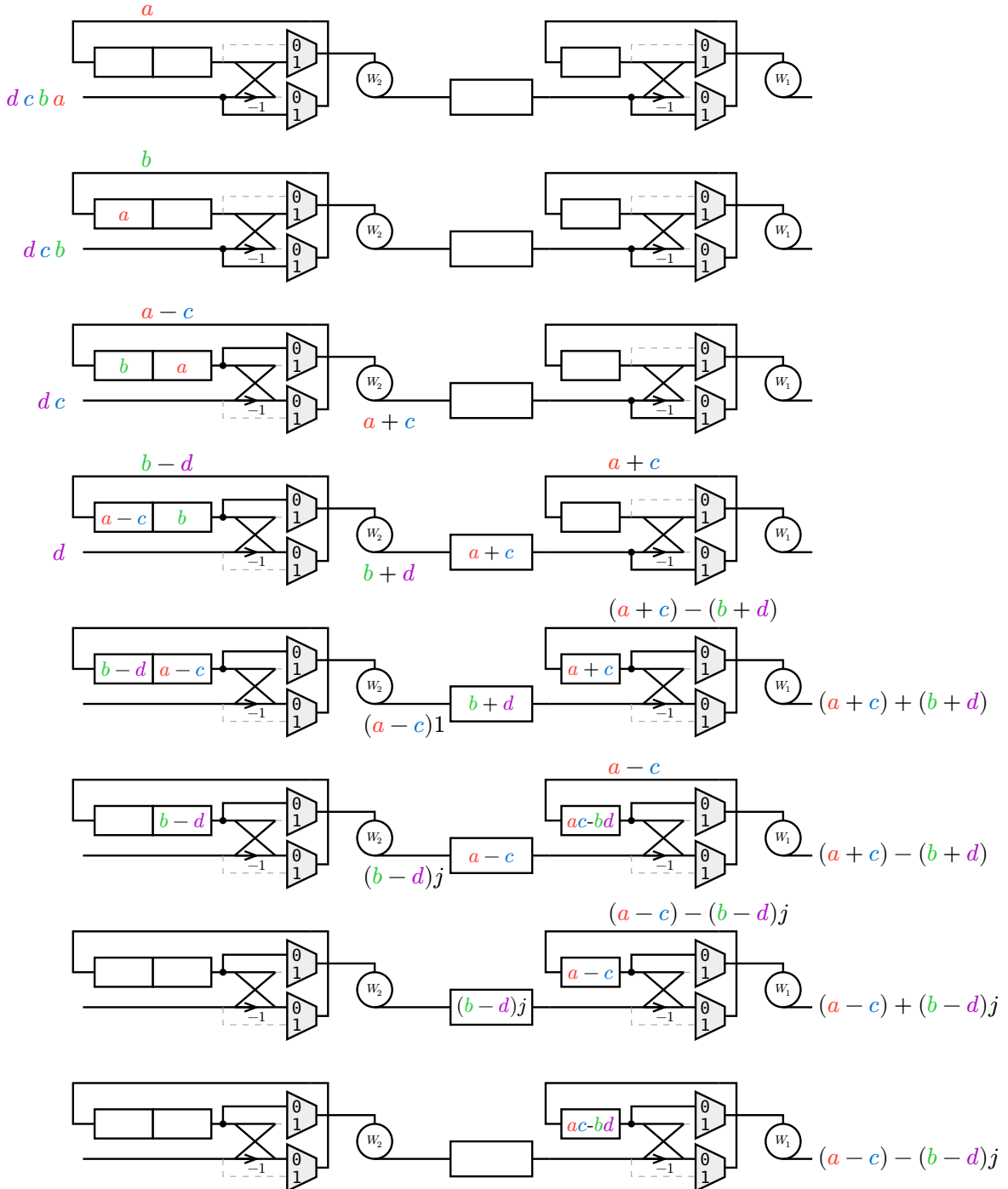
Figure 3.13: Steps involved in a 4 point R2SDC algorithm
