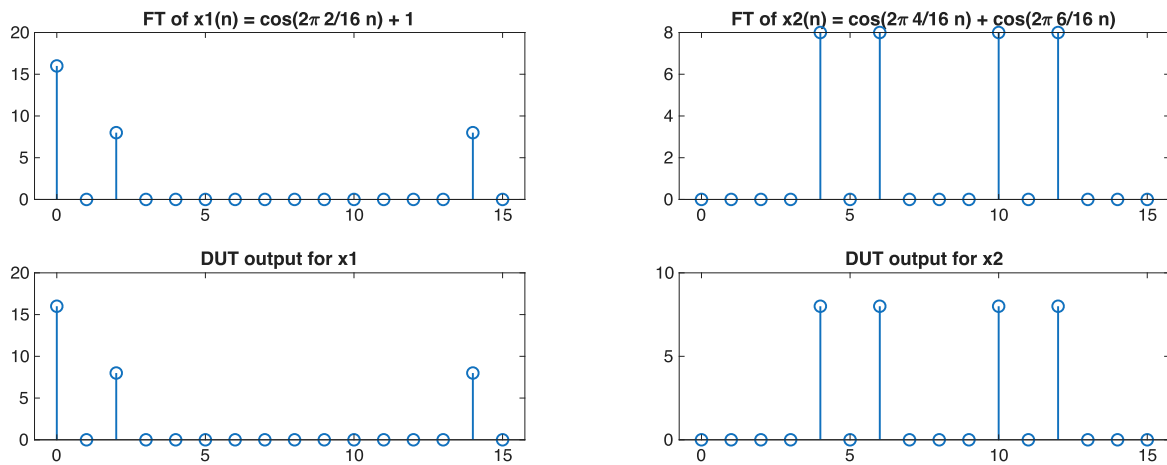
Figure 3.17: Comparison of output of FFT in MATLAB and simulation
